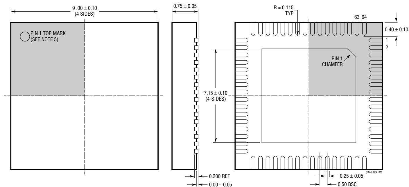
RECOMMENDED SOLDER PAD PITCH AND DIMENSIONS
